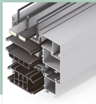
• Technoform Thermal insulating strip
